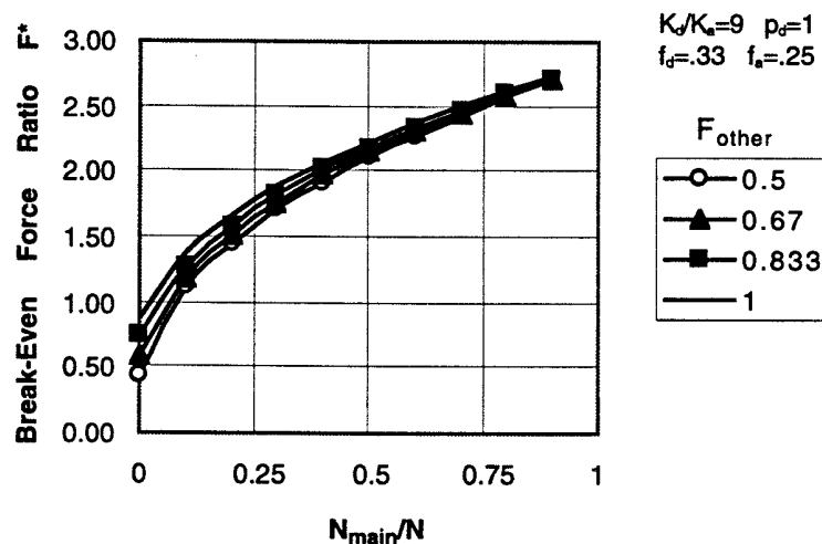
Figure 3—Break-Even Ratio Versus Force Ratio and N_{main}/N for Canonical Case
